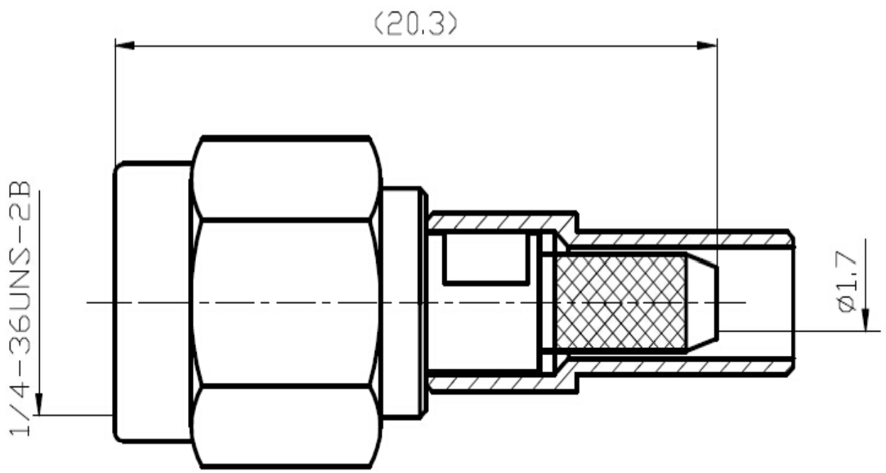
SMA-JC-316P
